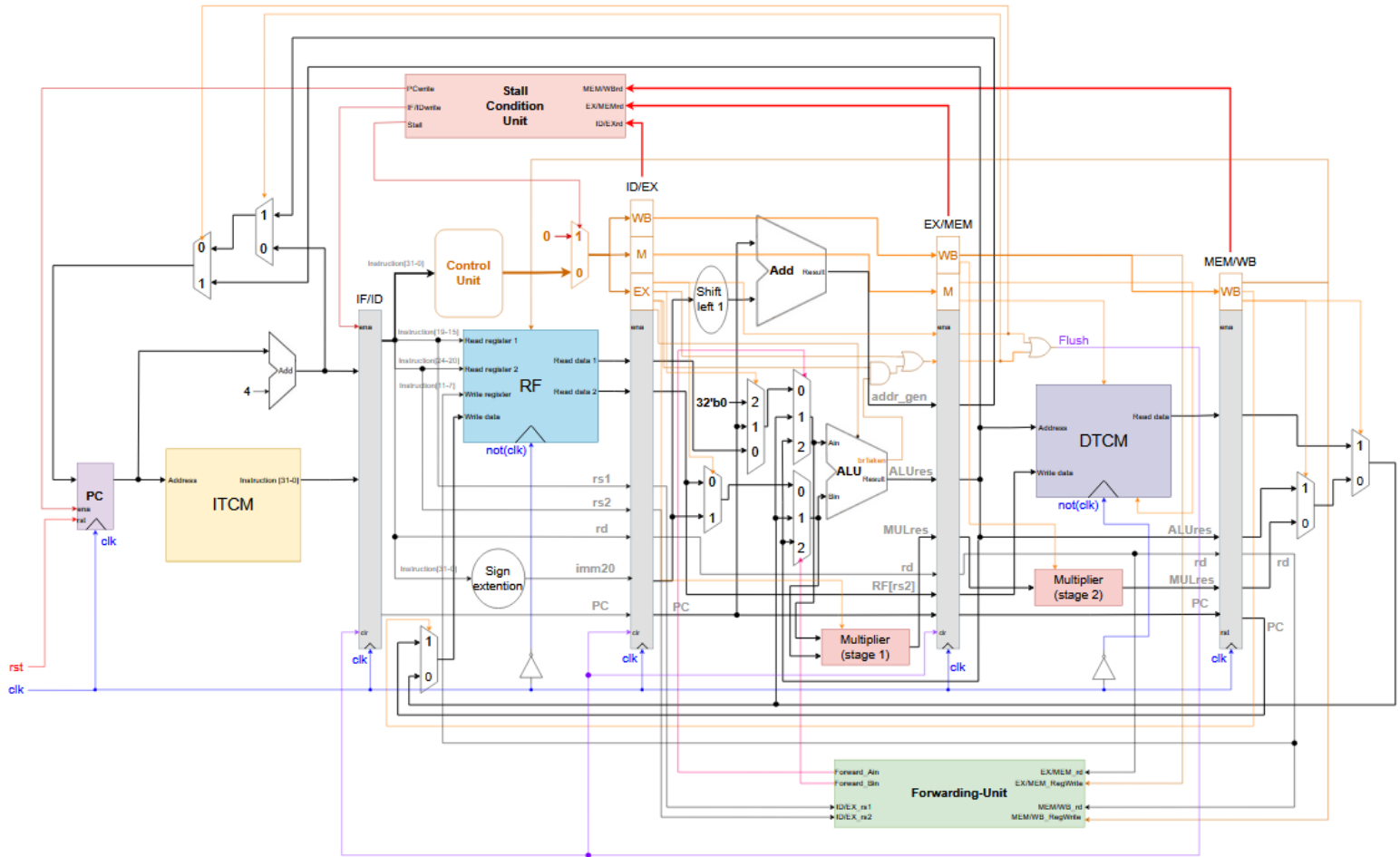
RISCV RV32I Single-Thread pipeline \mu Architecture (supports the base Integer unprivileged ISA) ©Hananya Ribo
