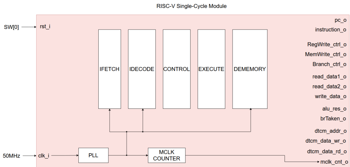
Figure 4: Single-cycle RV32I uArchitecture top entity
