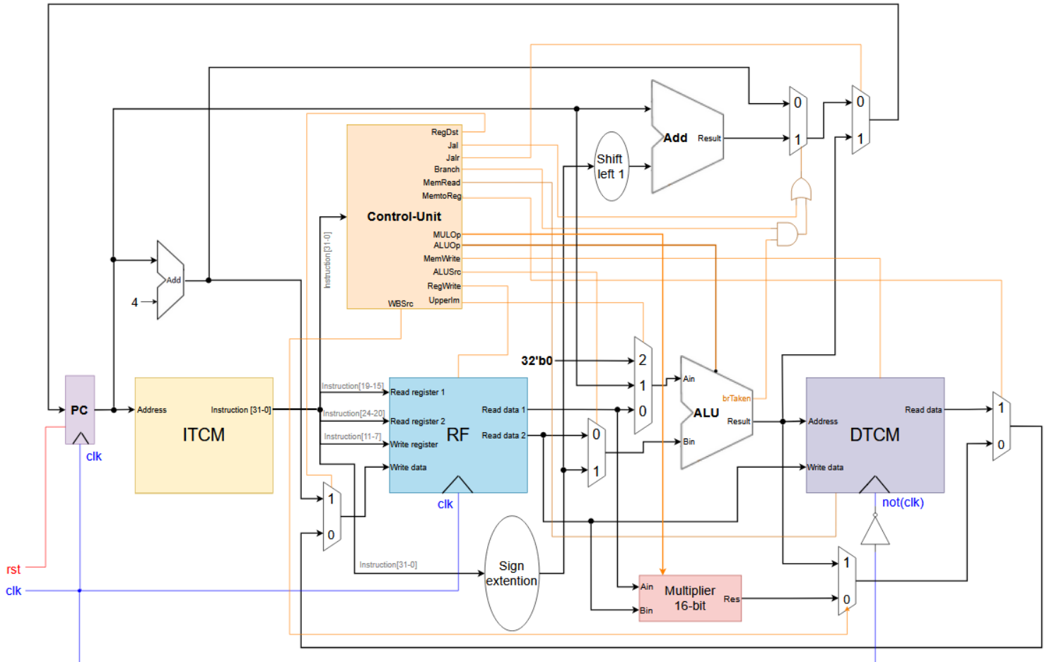
Figure 5: Single-cycle RV32IM (MULDIV partial) uArchitecture
